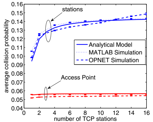
Fig. 9. Unfairness between AP and stations using saturated TCP traffic on the downlink.
