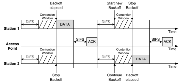
Fig. 1. Medium access example for DCF stations.
