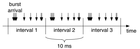
Fig. 5. Phase pattern illustration of voice traffic.
