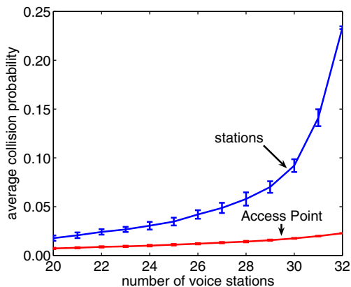
Fig. 10. Unfairness between AP and stations with a TXOPLimit of 1504 \mu\text{s} .
