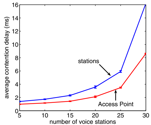
Fig. 11. Contention delay unfairness between Access Point and stations using a TXOPLimit of 1504 \mu\text{s} .
