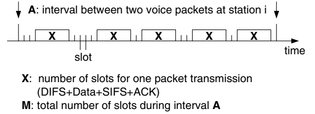
Fig. 6. Parameter illustration of the analytical model.
