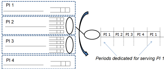
Fig. 1 Cycle-based scheduler for creating virtual links
