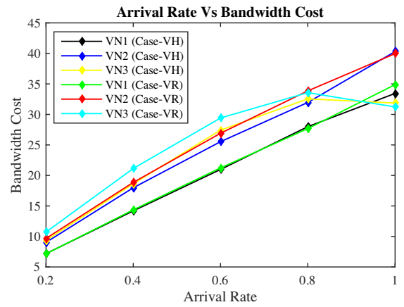
Fig. 7. Bandwidth Cost for each VN: Case-VH vs. Case-VR
