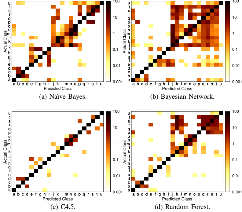
Figure 2: Confusion matrices (L3, percentage accuracy, log scale) for dataset D_5 and 10-fold validation (see Tab. I for class labels).
