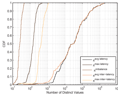
Fig. 2: Empirical CDFs of the number of distinct function values per problem instance for each objective function.
