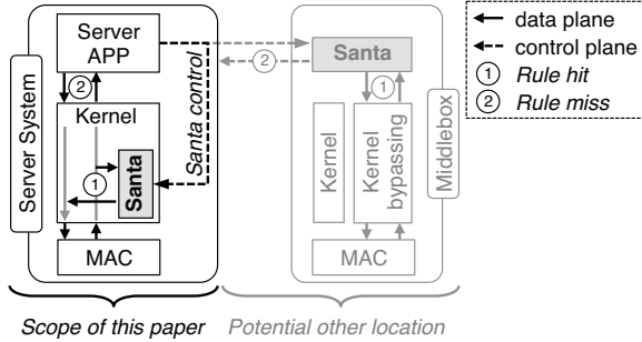
Fig. 1: Example execution positions of Santa: in-kernel (the focus of this paper) and in middleboxes (e.g., accelerated with kernel bypassing techniques such as DPDK or netmap).
