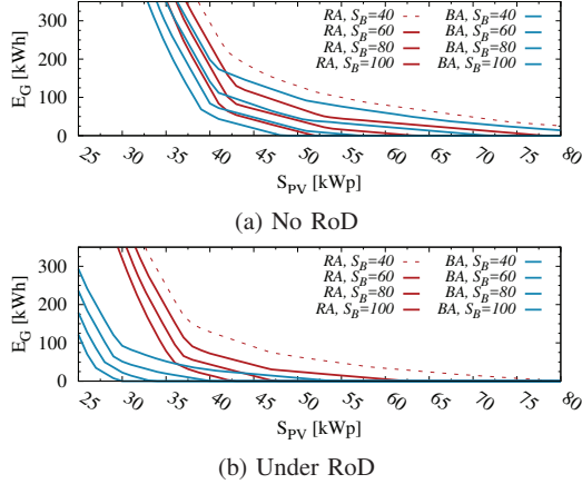
Fig. 4: Yearly grid energy, E_G , versus S_{PV} in Residential and Business area (RA and BA), for different storage sizes.
